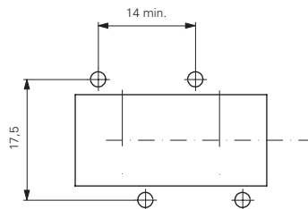
2 channel unit
