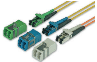
F-3000™ Duplex
