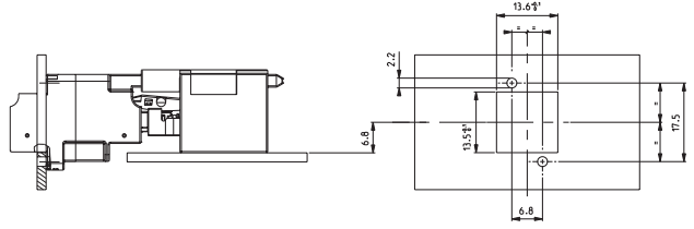
2 channel unit
